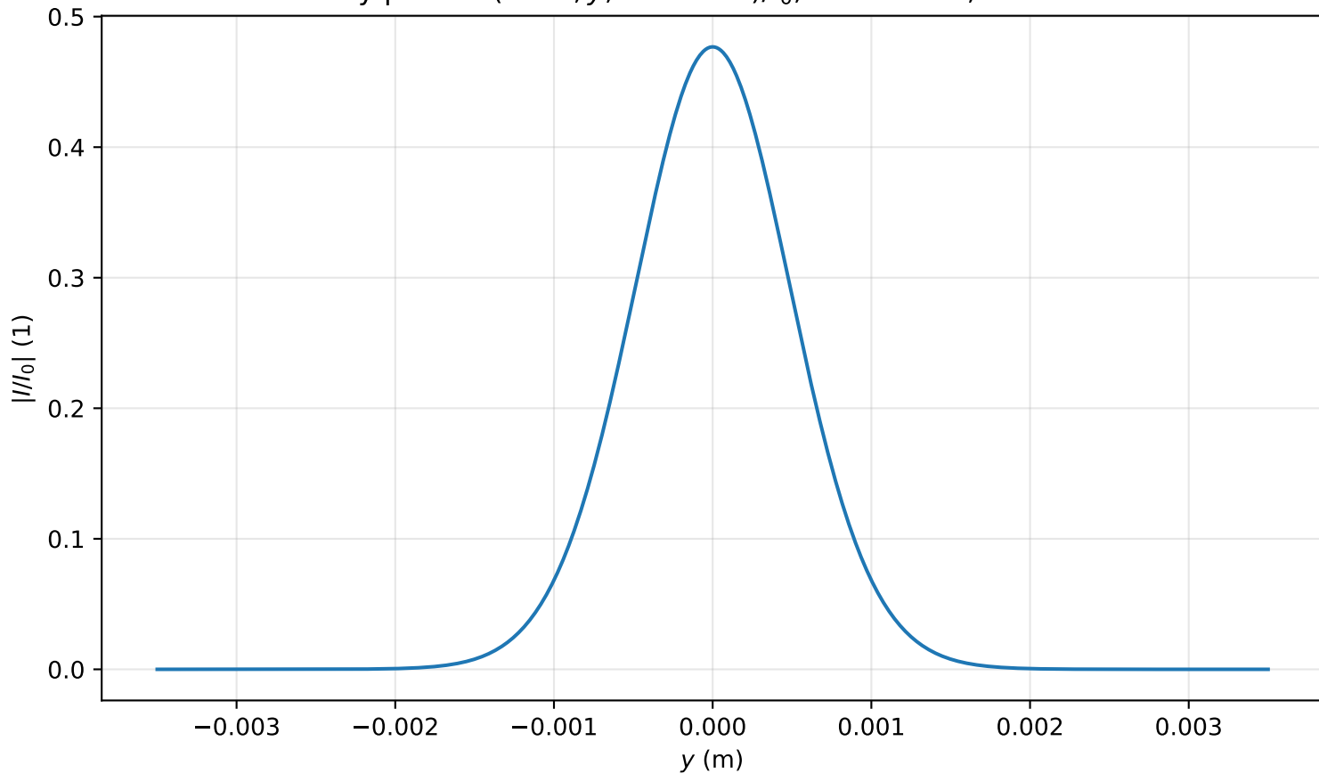
Intensity profile I(x=0, y, z=2.468)/I_0 , P_{in}=0.2P_{cr} , artificial time
